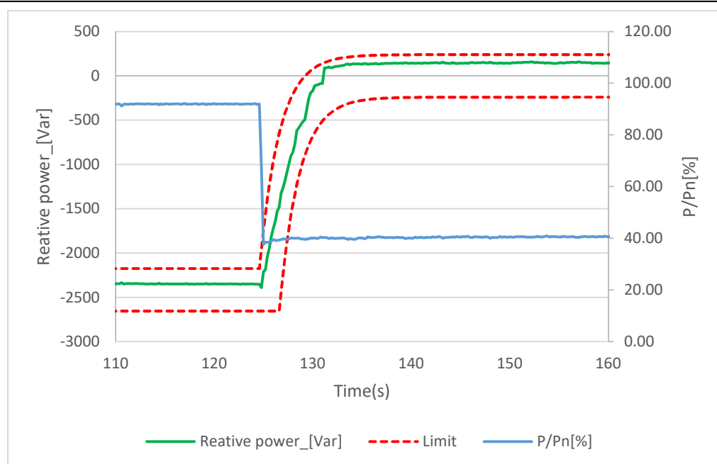
Graph of Test d): 100% to 40% P E max
